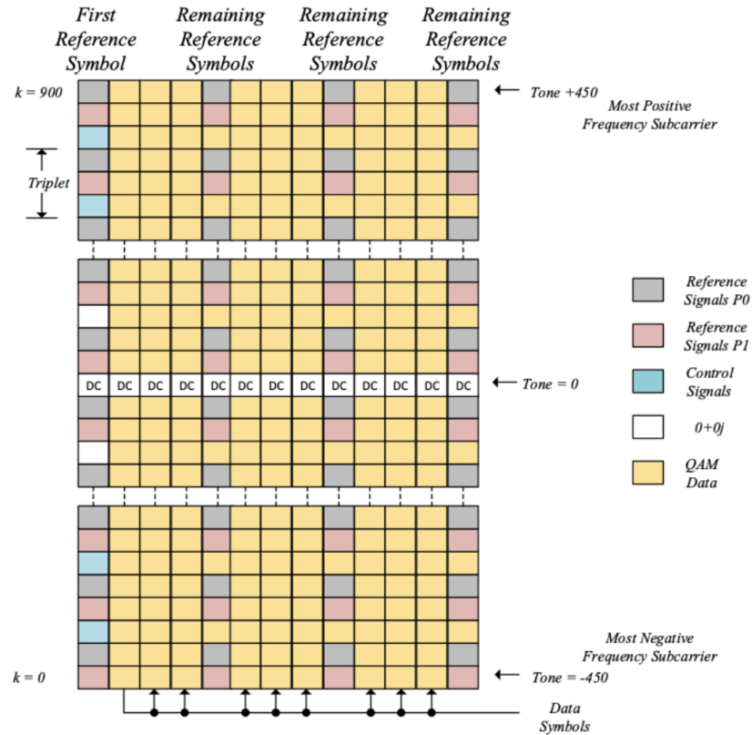
Figure 23: Reference Grid for the 20MHz Bandwidth Case and Subcarrier Spacing of 20KHz
